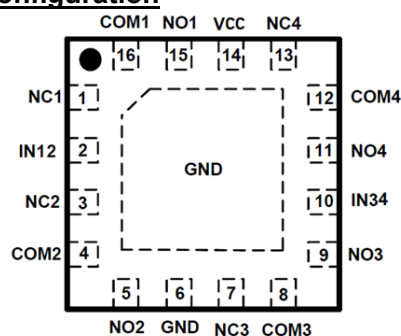
TOP View QFN3x3-16L
