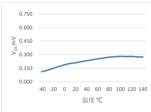
V_{OS} vs. Temperature
