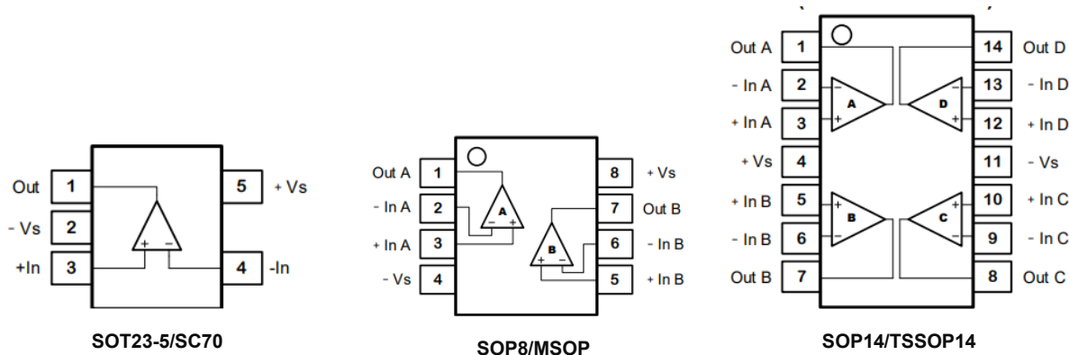
Figure 1. Pin Assignment Diagram
