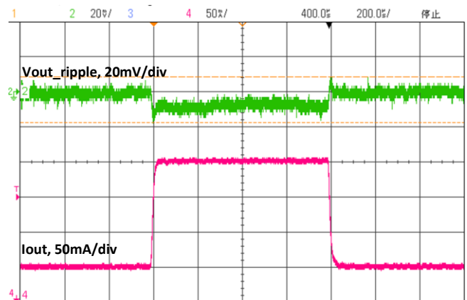
Load Transient Response (Vin=5V, Vout=3.3V, Iout=150-300mA)
