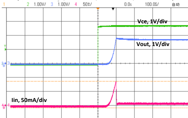
CE Chip Enable Response (CE=0V to 2.8V, Vin=2.8V, Vout=1.8V, Iout=10mA)
