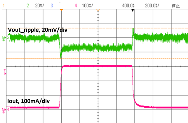
Load Transient Response (Vin=5V, Vout=3.3V, Iout=10-300mA)
