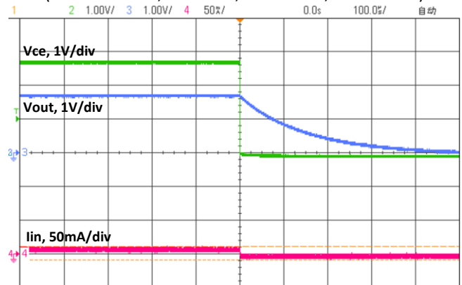
CE Chip Enable Response (CE=2.8V to 0V, Vin=2.8V, Vout=1.8V, Iout=10mA)
