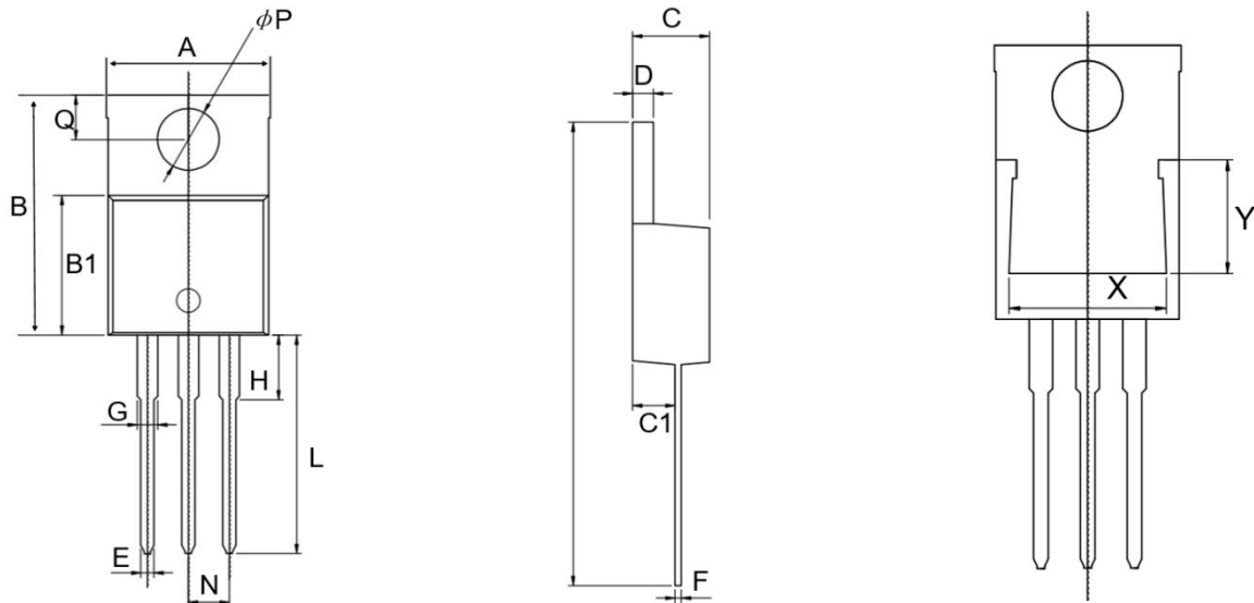
TO-220 Package
