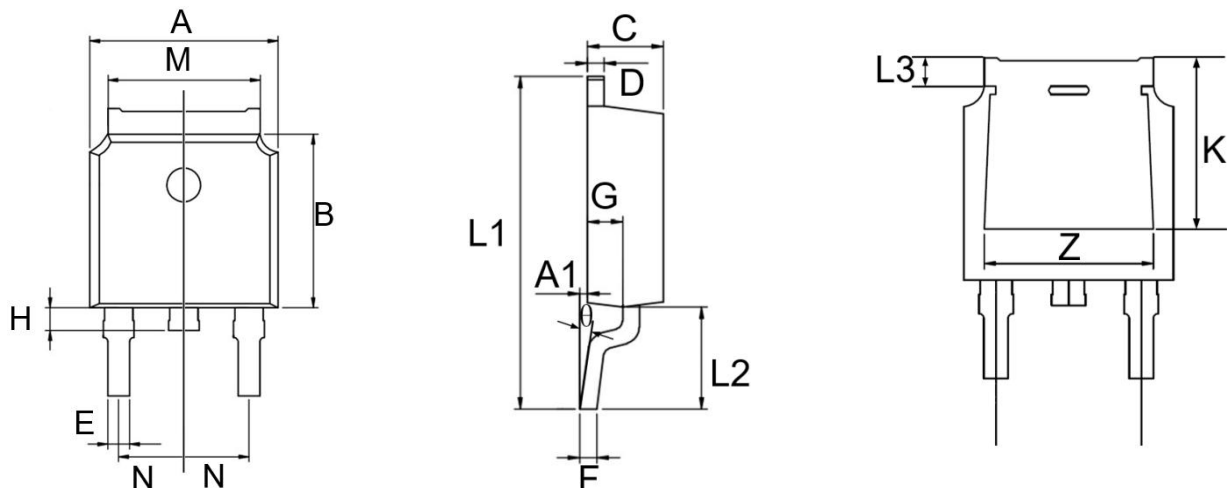
TO-252 Package
