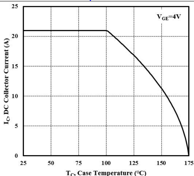
Figure 6. DC Collector Current vs Case Temperature
