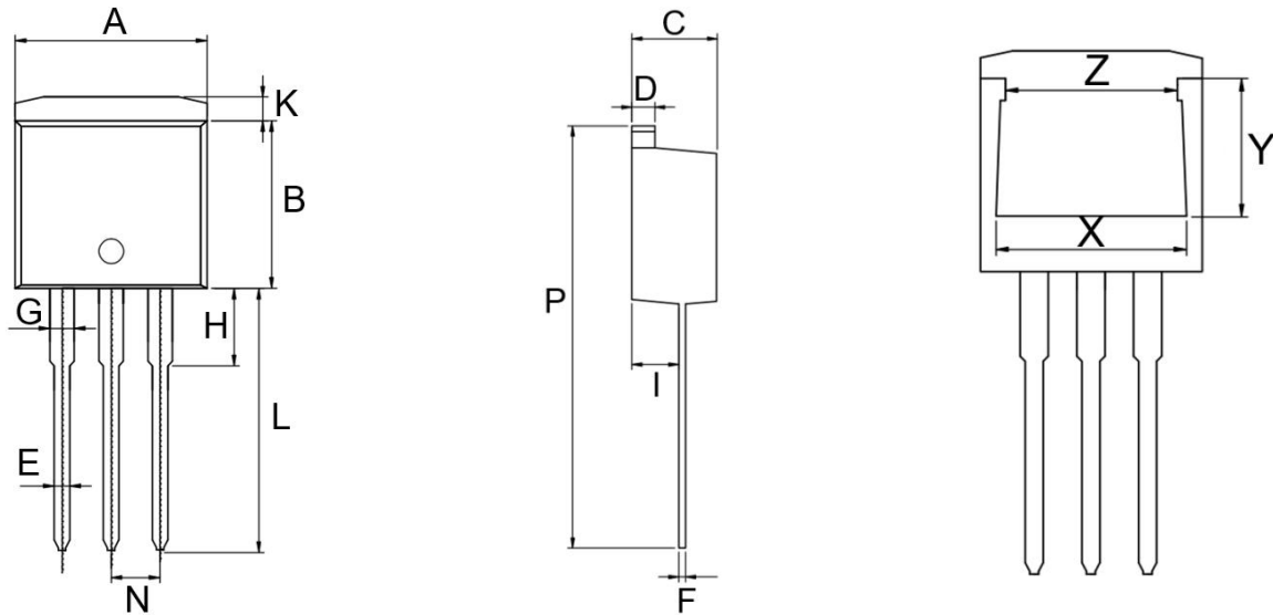
TO-262 Package
