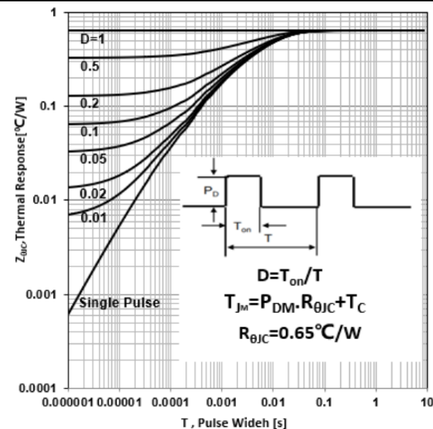
Figure 20. Diode Transient Thermal Impedance vs Pulse Width (TO247/TO3PF/TO3PN)
