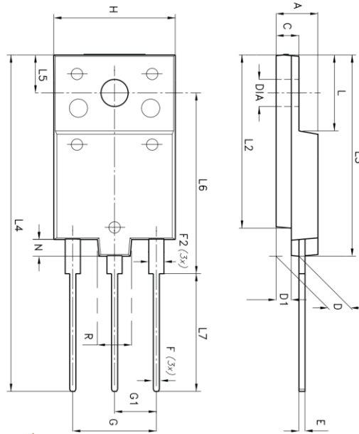
TO-3PF Package
