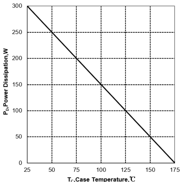
Figure 2. Power Dissipation vs Case Temperature for TO247/TO3PF/TO3PN
