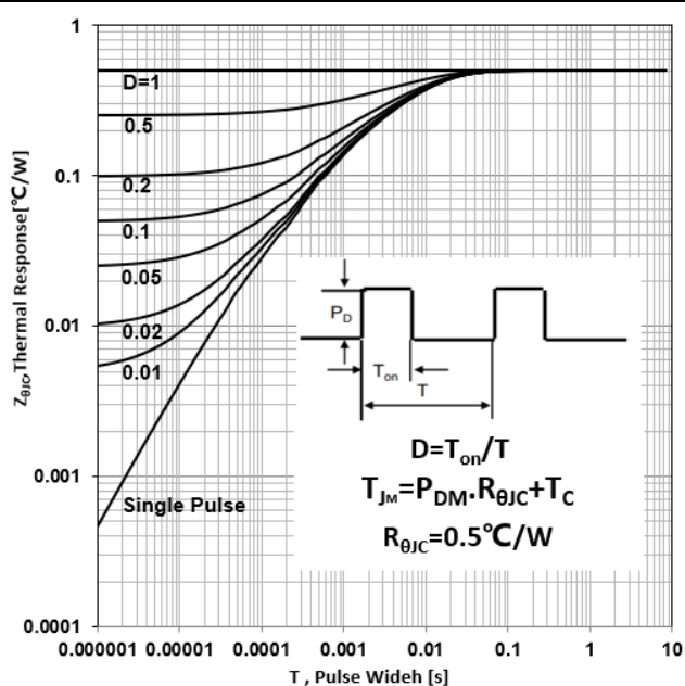
Figure 19. IGBT Transient Thermal Impedance vs Pulse Width(TO247/TO3PF/TO3PN)
