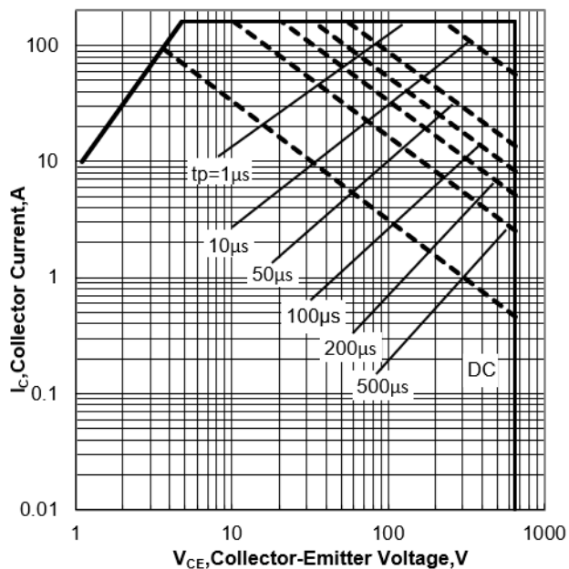
Figure 1. Forward Bias Safe Operating Area for TO247/TO3PF/TO3PN
