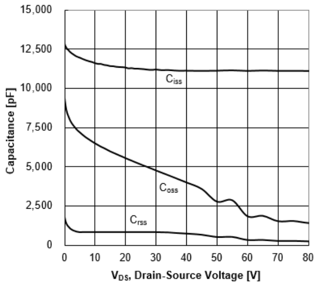
Figure 12. Capacitance Characteristics
