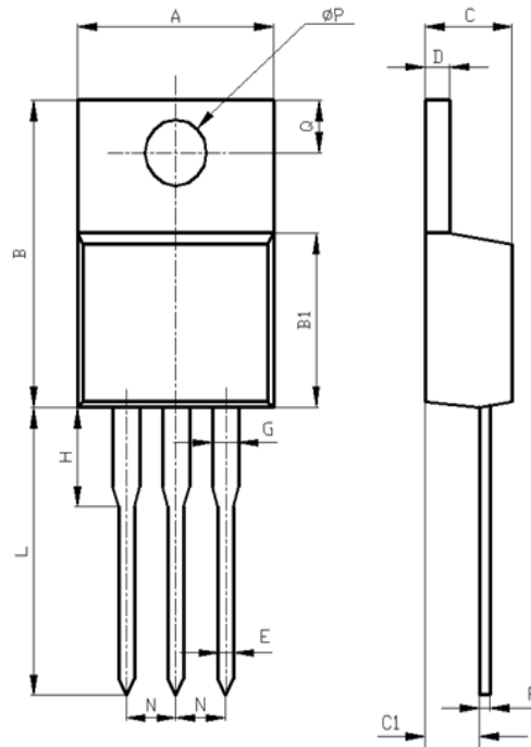
TO-220
