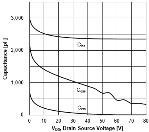
Figure 12. Capacitance Characteristics
