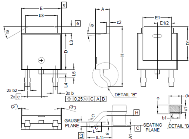
TO-252 Package
