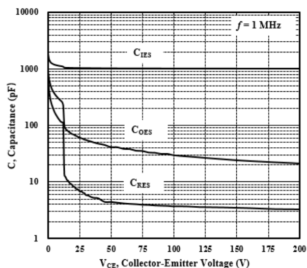
Figure 14 Capacitance vs Collector to Emitter Voltage
