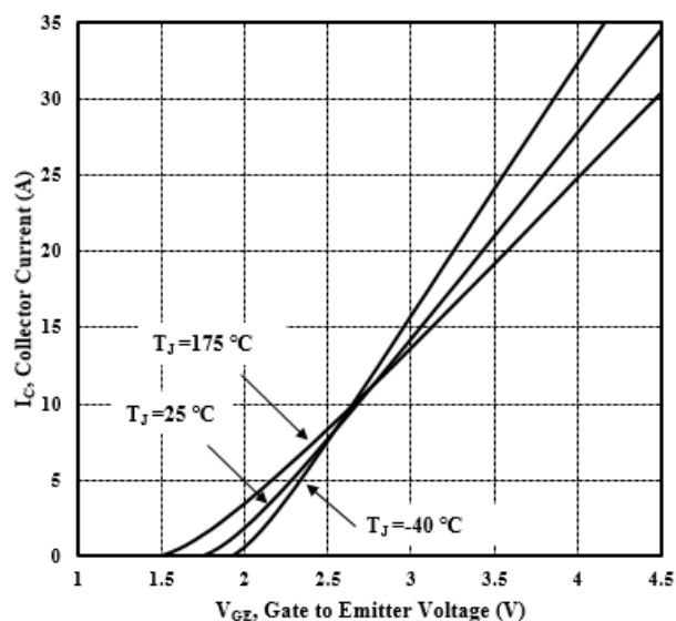
Figure 13 Transfer Characteristics
