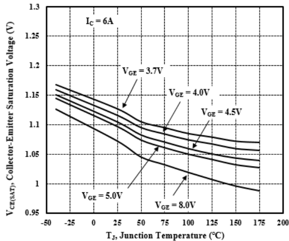
Figure 1 Collector-Emitter Saturation Voltage vs Junction Temperature
