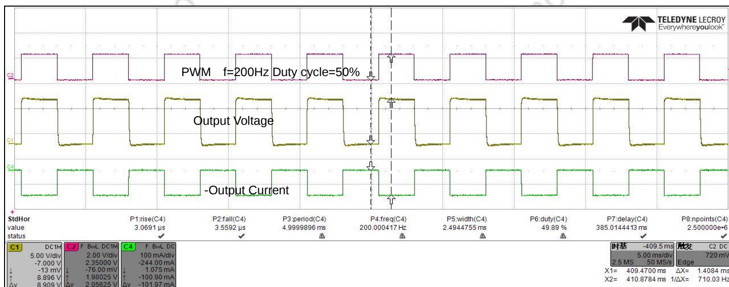
Figure 10. PWM Dimming
