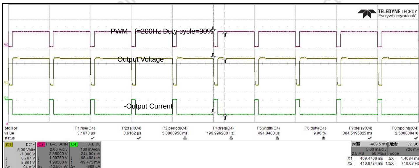
Figure 11. PWM Dimming
