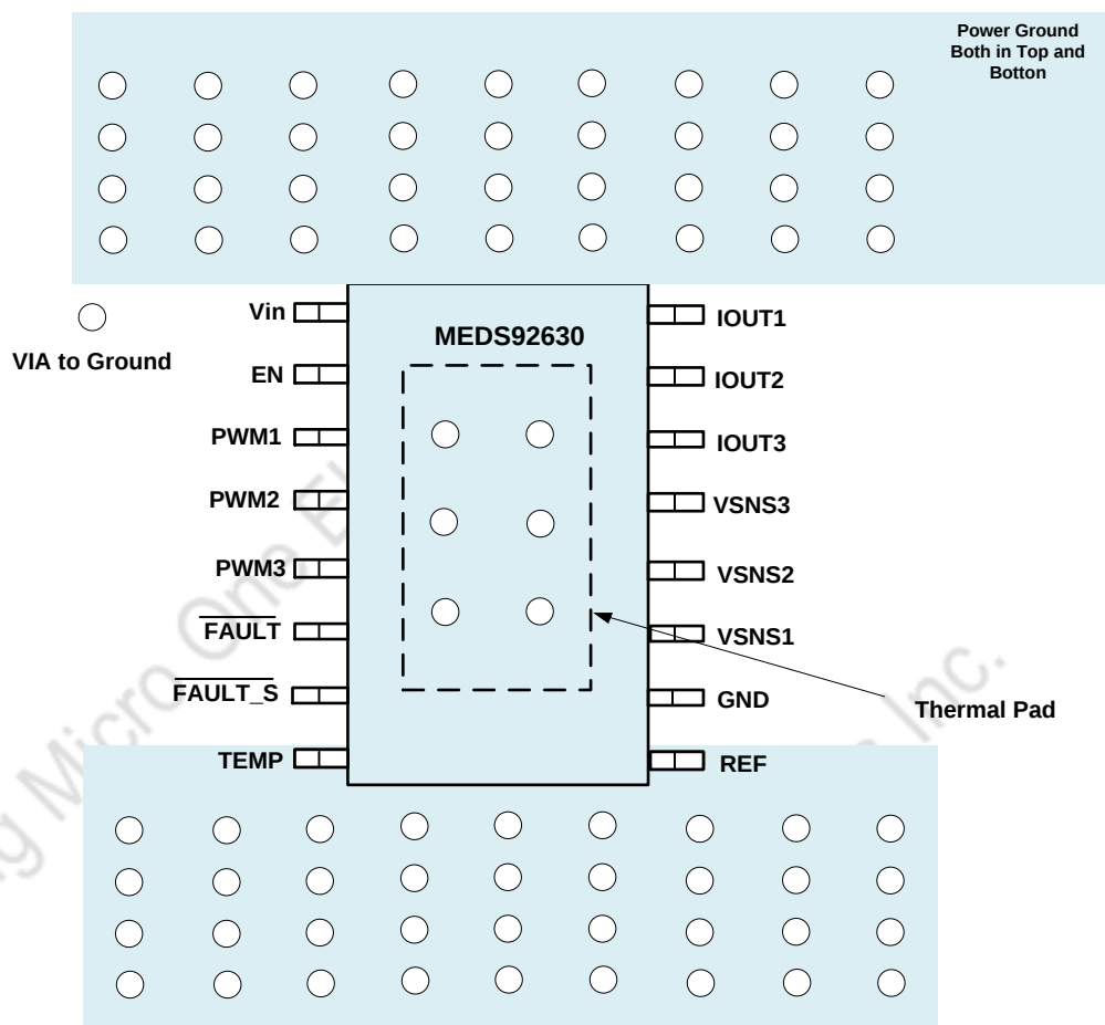
Figure 22.MEDS92630 Board Layout
