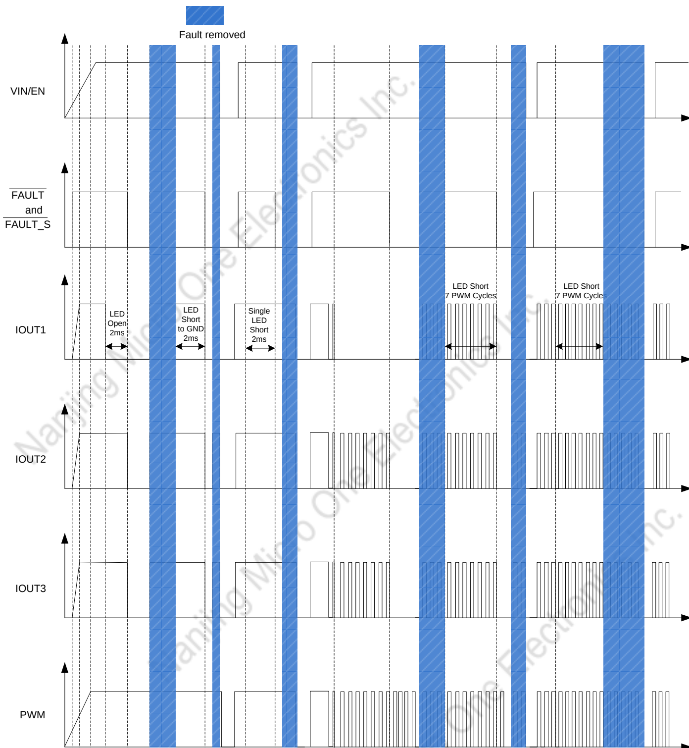
Figure 17. Detailed Timing Diagram
