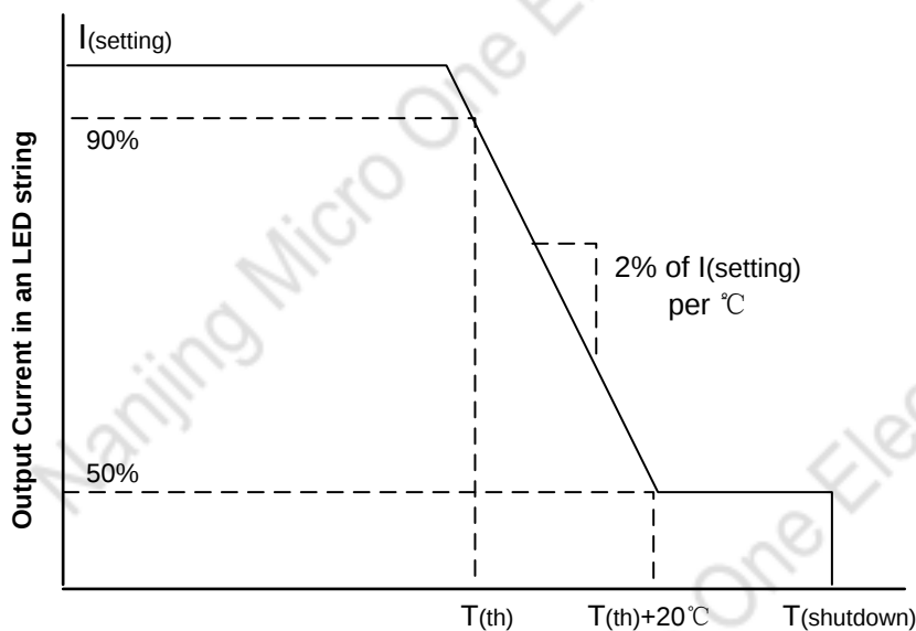
Figure 20. Thermal Foldback
