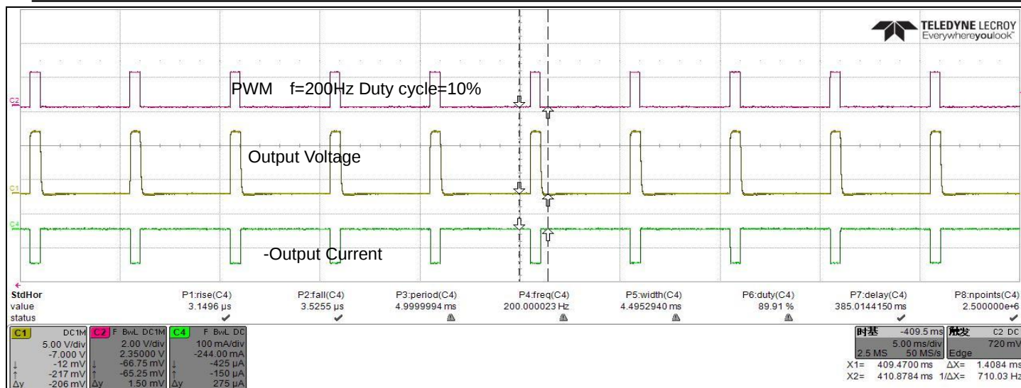
Figure 9. PWM Dimming
