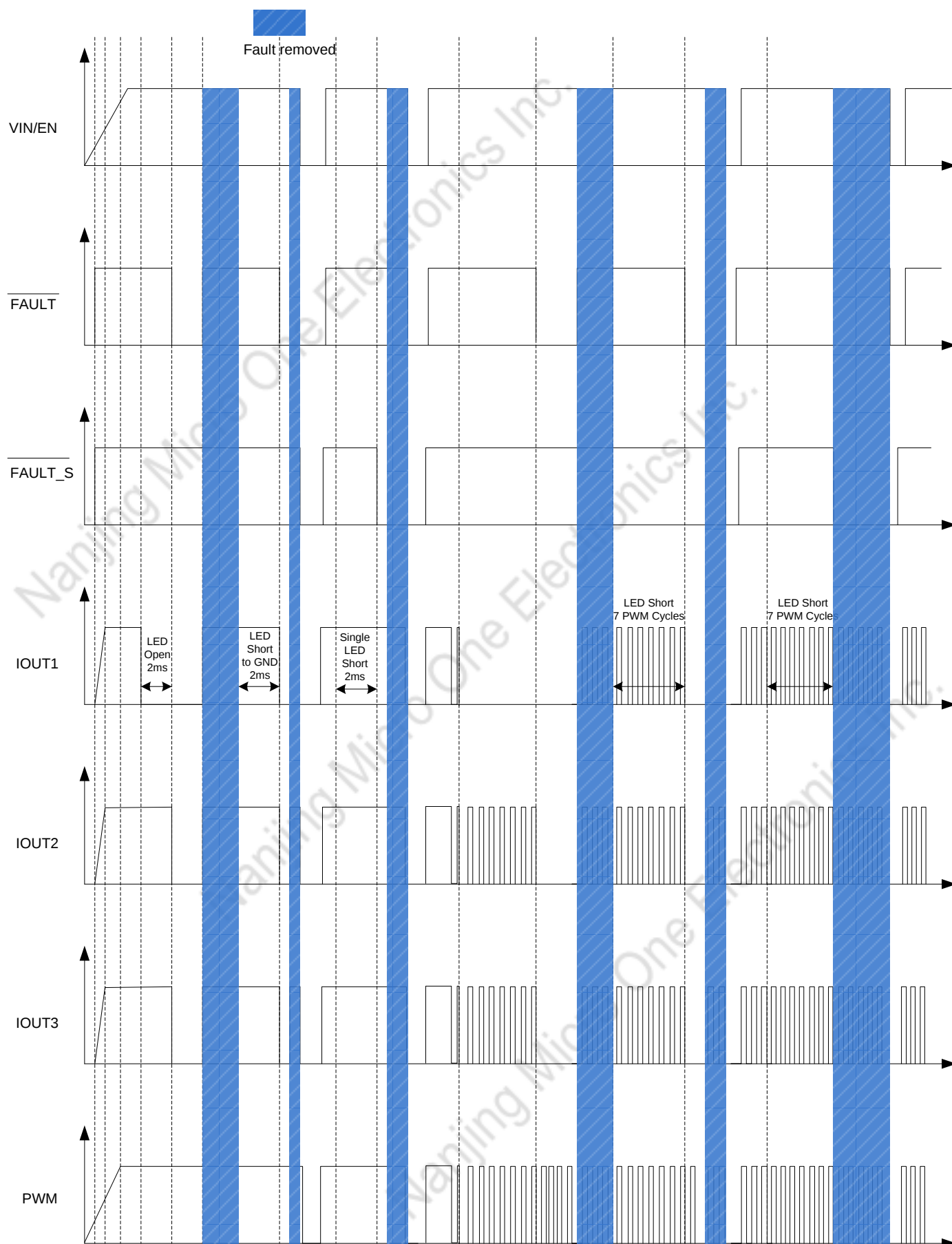
Figure 15. Detailed Timing Diagram
