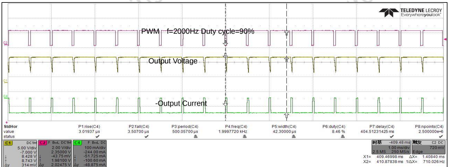
Figure 14. PWM Dimming
