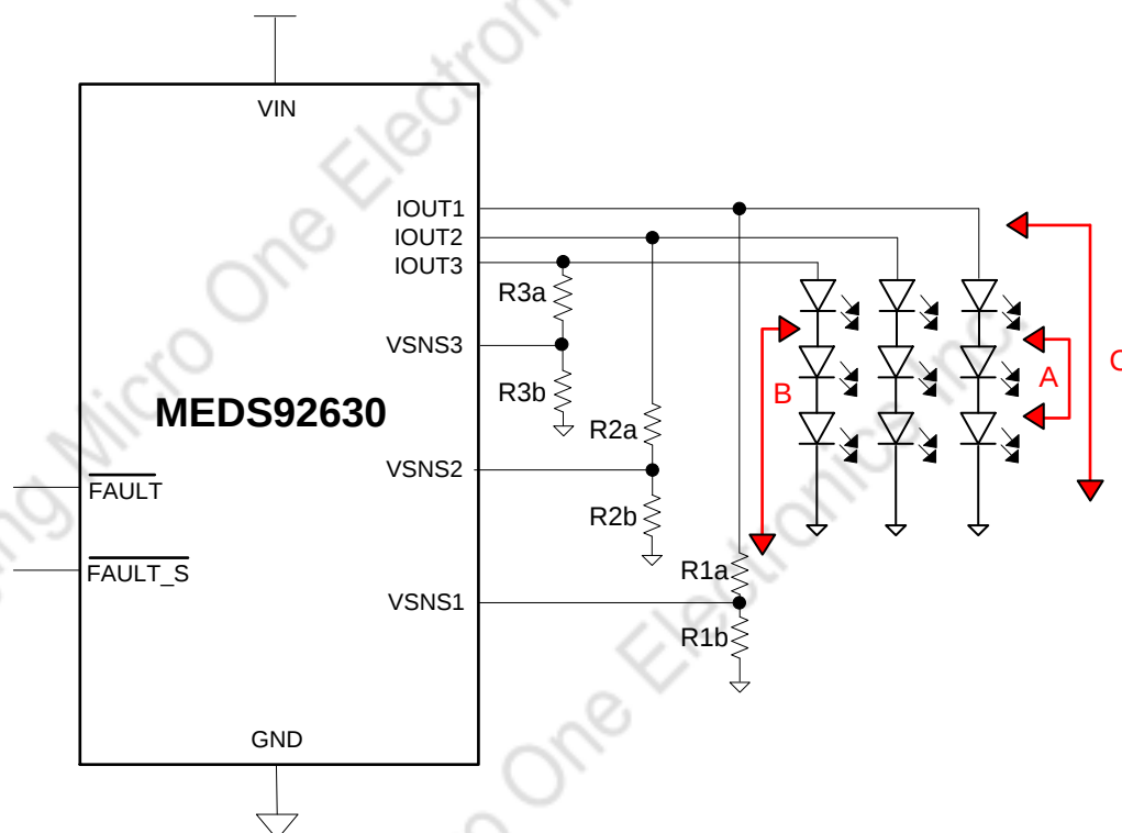
Figure 18. Short-Circuit Cinditions
